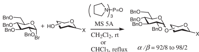
Scheme 1. Glycosylation of several acceptors with 2,3,4,6-tetra- O -benzyl-D-glucopyranosyl bromide promoted by tri(1-pyrrolidino)phosphine oxide.
