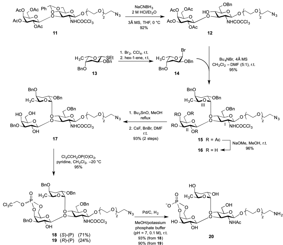
Scheme 2. Synthesis of the Spacer-Equipped, Phosphorylated Trisaccharide 20
