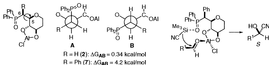
Fig. 1. Newman projection in terms of C5–C6 bond of catalysts 2 and 7 and working model of the transition state with 7
