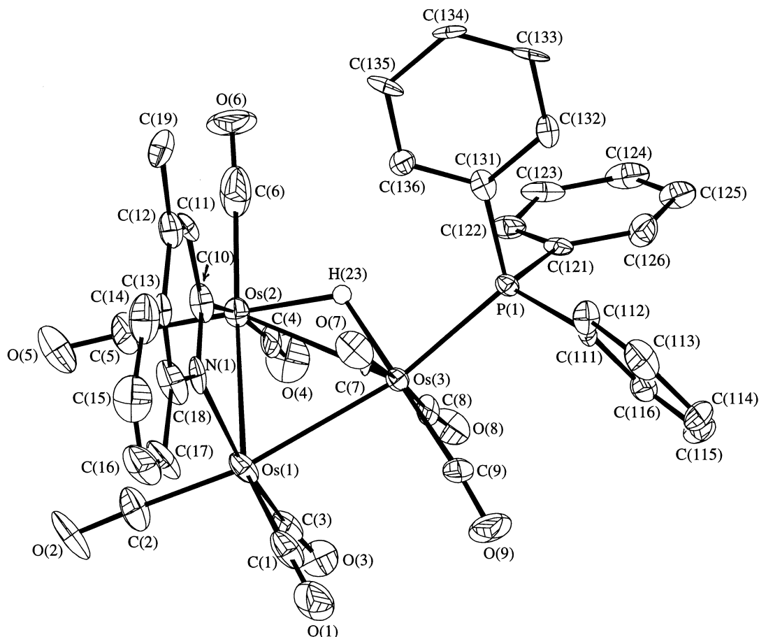
Fig. 2. Solid state structure of [(\mu\text{-H})\text{Os}_3(\text{CO})_9\{\mu\text{-}1,2\text{-}\eta^2\text{-C}_9\text{H}_5(\text{CH}_3)\text{N}\}(\text{PPh}_3)] 10 showing the atom labelling scheme. Thermal ellipsoids are drawn at 50% probability level. The ring hydrogen atoms are omitted for clarity.
