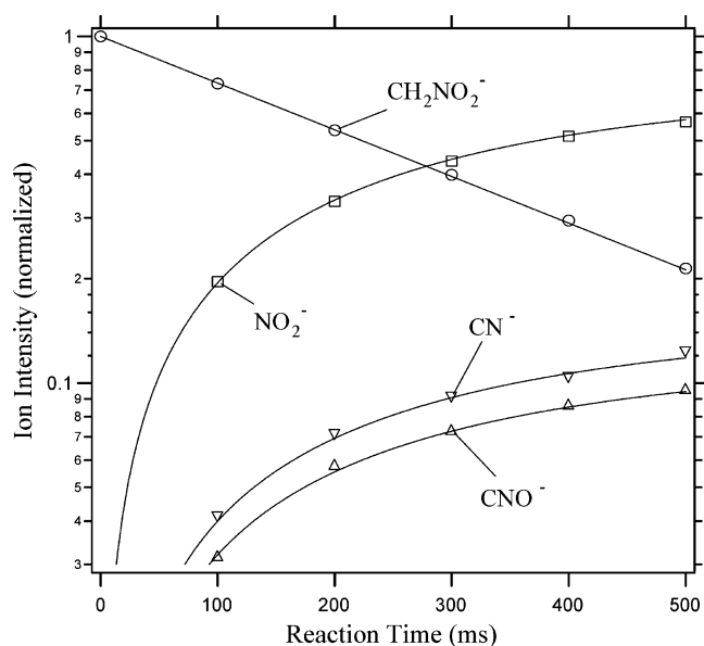
Figure 4. Semilogarithmic plot of the anion intensities vs reaction time. The solid lines are the curve fittings assuming the rate constant as 3.1 \text{ s}^{-1} and the branching ratios to generate NO 2 − , CN − , and CNO − as 73, 15, and 12%, respectively.
