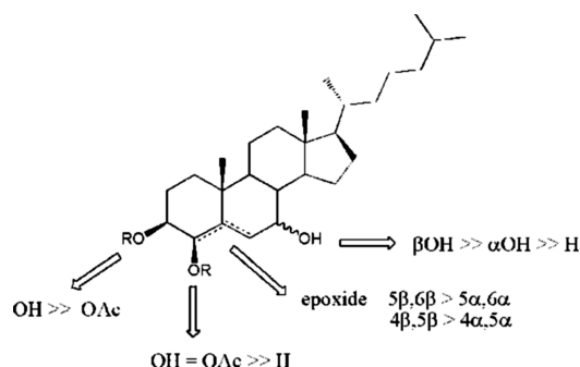
Figure 2. Graphical depiction of the SAR for cell cytotoxicity based on the IC_{50} results.
