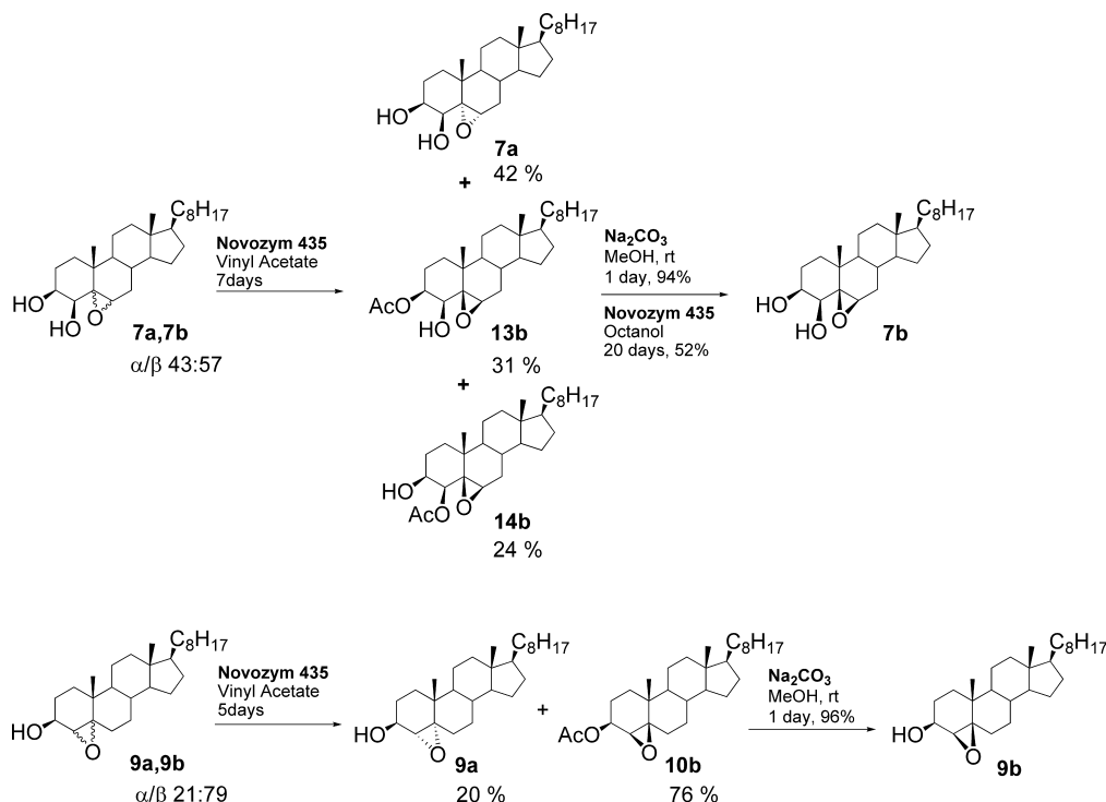
Scheme 4. Chemoenzymatic Discrimination of 4,5- and 5,6-Epoxycholestanes
