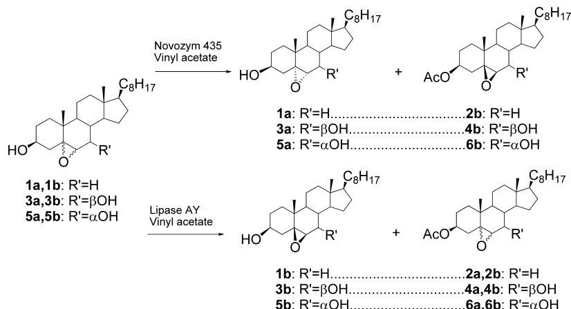
Scheme 4. Chemoenzymatic Discrimination of 4,5- and 5,6-Epoxycholestanes
