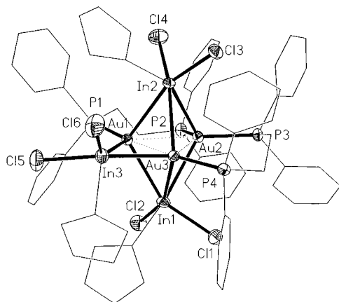
Figure 4. Molecular structure of (dppe)_2Au_3(InCl_2thf)_3 (hydrogen atoms omitted for clarity). 11
