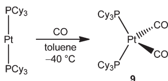
Scheme 4. Synthesis of the Platinum Dicarbonyl Complex 9
