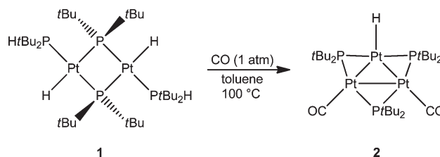
Scheme 1. Synthesis of the Triangular Cluster 2
