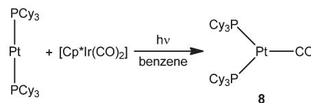
Scheme 3. Formation of the Platinum Monocarbonyl Complex 8
