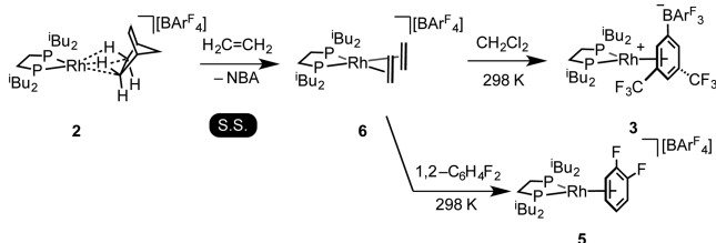
Scheme 3. Formation of Complex 6 in the Solid-State and the Decomposition Reactions That Occur in Solution When Excess Ethene Is Not Present
