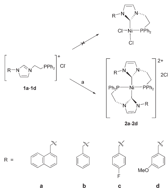
Scheme 1. Synthesis of [\text{Ni}(\text{L})_2]\text{Cl}_2 . Conditions: a) For \mathbf{2a} and \mathbf{2c} only \text{NiCl}_2/\text{NaOAc} ; for \mathbf{2a-2d} \text{Ni}(\text{OAc})_2 .
