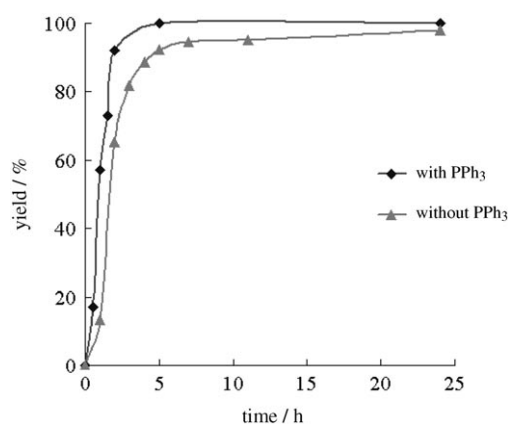
Figure 7. Comparison of the time/yield characteristics of 2a with and without the addition of \text{PPh}_3 in the cross-coupling of phenylboronic acid and 4-chlorotoluene.
