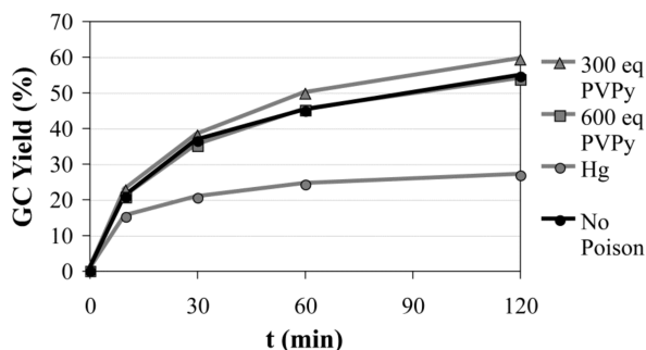
Figure 4. Poisoning tests for the catalytic system \text{Pd}_2(\text{dba})_3 \cdot \text{CHCl}_3/\mathbf{1} in reaction 5.
