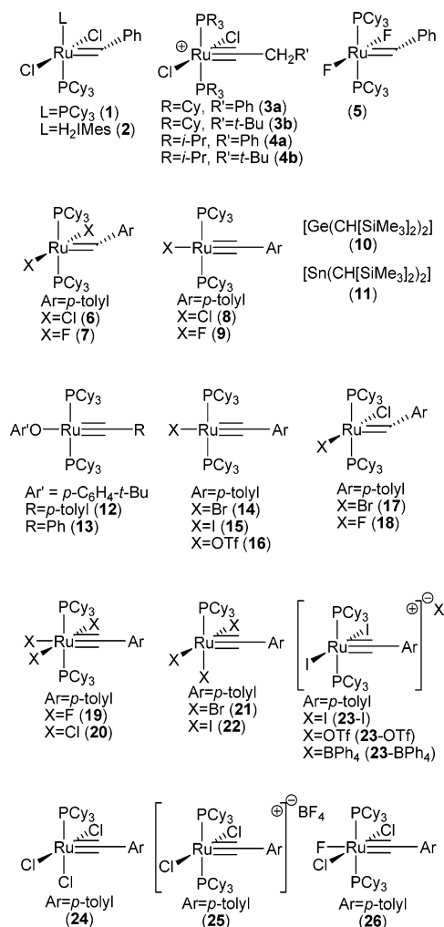
Chart 1. Numbered Compounds
