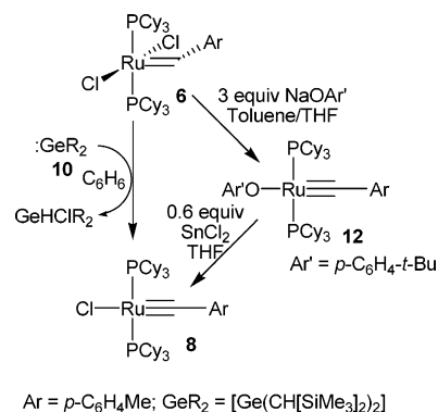
Scheme 1. Synthesis of Square-Planar Mono-chloride Benzyldiene Complex
