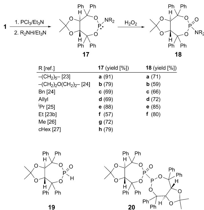
Scheme 3. Preparation of Phosphoramidites 17 , Phosphoroxamidites 18 , and of the Phosphite 19 , and Isolation of the P^V/P^{III} Derivative 20 from TADDOL, PCl_3 , R_2NH , and H_2O_2
