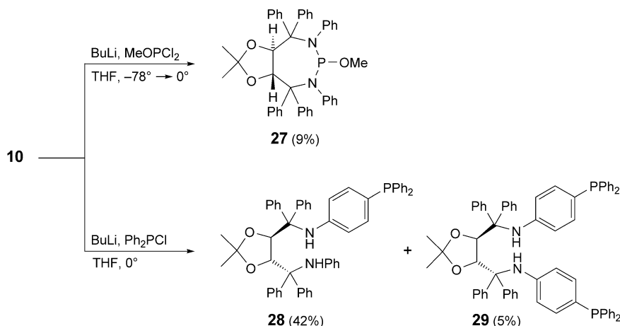
Scheme 5. Reactions of the TADDAMIN 10 with a Chloro- and Dichlorophosphine Derivative. Besides the isolated and characterized products 27–29 many non-identified compounds were present in the crude reaction mixtures; from the reaction with \text{Ph}_2\text{PCl} , 30% of starting material 10 was recovered.
