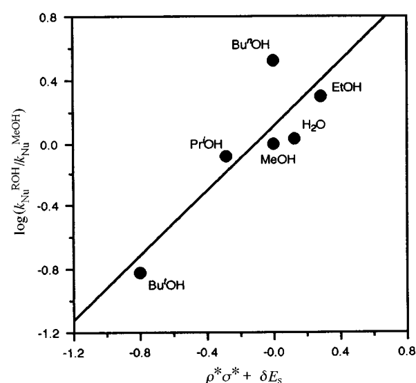
Fig. 6 Correlation of \log(k_{Nu}^{ROH}/k_{Nu}^{MeOH}) with \rho^* \sigma^* + \delta E_s in Taft's dual-parameter equation.
