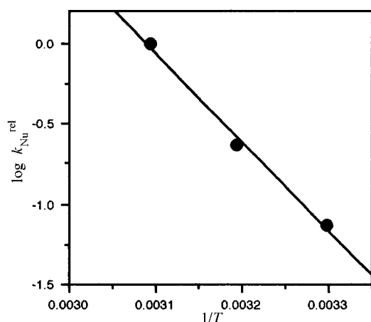
Fig. 4 The Arrhenius plot for the ionic reaction of radical cation BP^{\bullet+} with EtOH.
