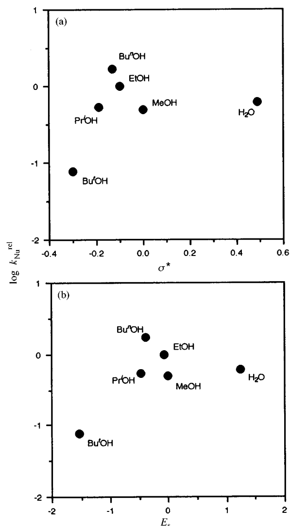
Fig. 5 Dependence of \log k_{Nu}^{rel} on the Taft's electronic parameter \sigma^* (a) and on the steric parameter E_s (b) of R in ROH.
