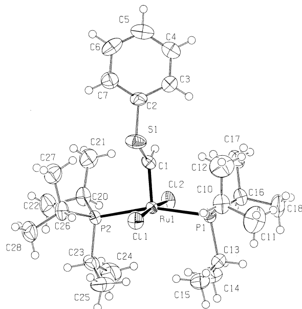
Fig. 1. ORTEP drawing of the molecular structure of [RuCl 2 (=CHSPh)(P i Pr 3 ) 2 ] ( 2a ) (thermal ellipsoids at 50% probability).
