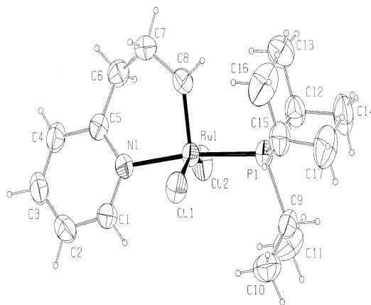
Fig. 2. ORTEP drawing of the molecular structure of [RuCl_2(=CHCH_2CH_2\text{-}C,N\text{-}2\text{-}C_3H_4N)(P'Pr_3)] ( 4a ) (thermal ellipsoids at 50% probability).
