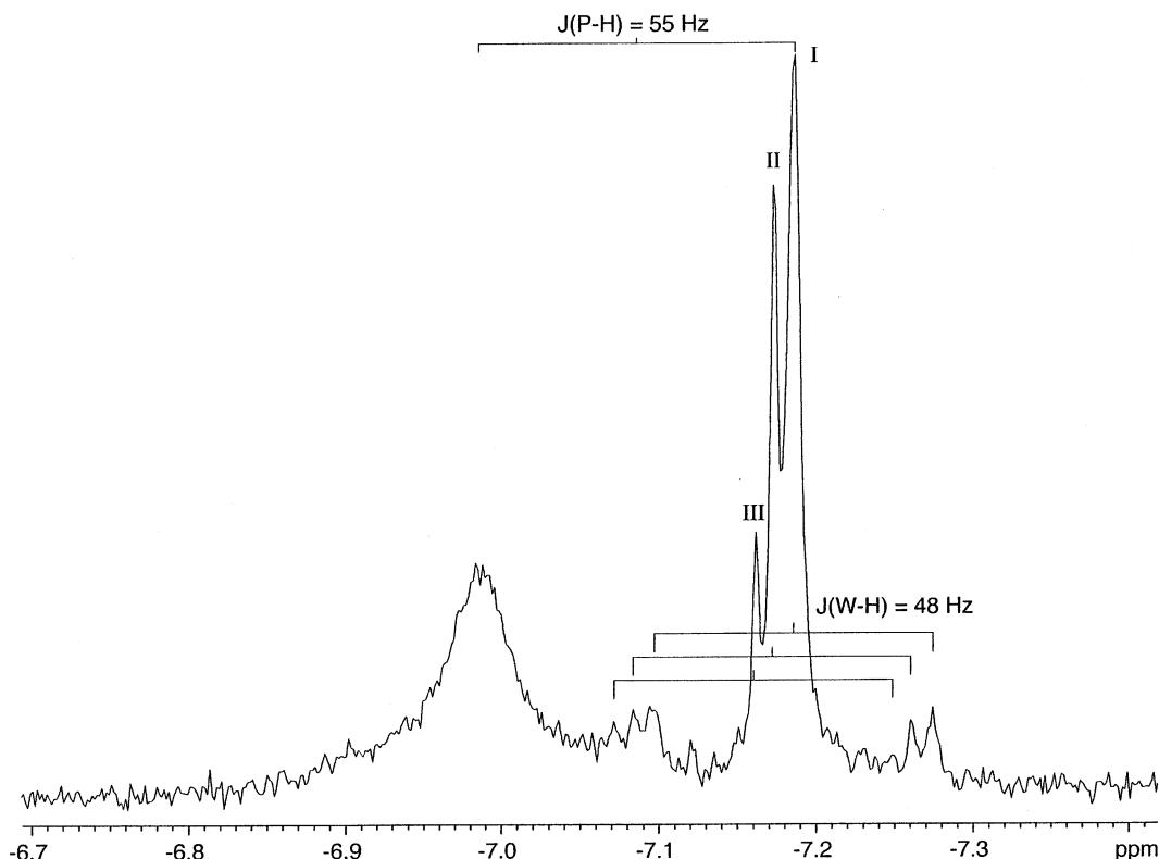
Fig. 3. Hydridic proton region of the ^1\text{H} -NMR (270 MHz) spectrum of a reaction mixture of 1 with \text{CCl}_4 in acetone- d_6 . (I) Complex 1 ; (II) cis - \text{FvW}_2(\text{CO})_4(\text{PPh}_2\text{Me})_2\text{HCl} ; (III) trans - \text{FvW}_2(\text{CO})_4(\text{PPh}_2\text{Me})_2\text{HCl} .
