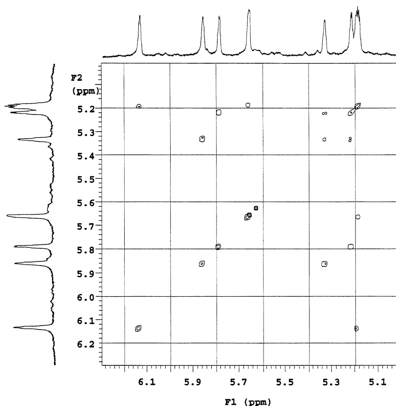
Fig. 1. COSY (500 MHz) spectrum of complex 2 in acetone- d_6 solution.
