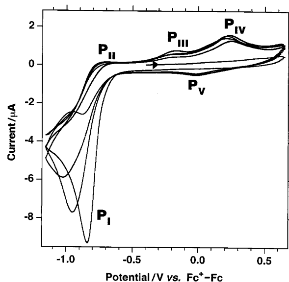
Fig. 4 Cyclic voltammogram (four cycles) of complex 4 in dcm-0.1 M [NBu 4 ][PF 6 ] at a freshly polished platinum-disc working electrode; scan rate = 100 mV s -1 and temperature = 295 K.
