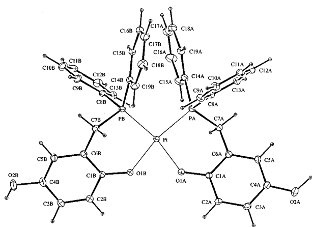
Fig. 1 An ORTEP 26 plot of cis -[Pt( O,P -PPh 2 thqH) 2 ] 2 . The thermal ellipsoids are drawn at the 10% probability level.
