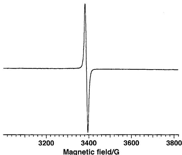
Fig. 9 The EPR spectrum of the product ( 6^{\bullet-} ) from reduction of complex 4 with cobaltocene (1 equivalent). Conditions: dmf glass, T = 77\text{ K} , \nu = 9.497\text{ GHz} .
