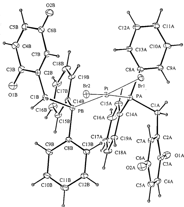
Fig. 2 An ORTEP plot of cis -[PtBr 2 (PPh 2 thq)] 2 4 . Details as in Fig. 1.
