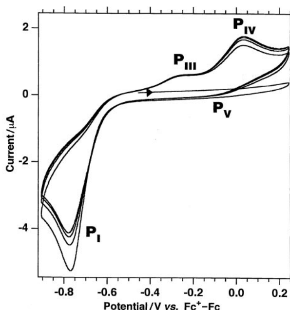
Fig. 5 Cyclic voltammogram (four cycles) of complex 4 in dmf-0.1 M [NBu 4 ][PF 6 ]. Other details as in Fig. 4.
