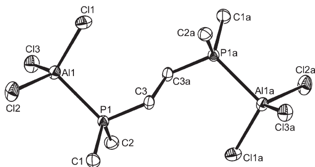
Fig. 5 The structure of centrosymmetric [(AlCl 3 ) 2 ( \mu -Me 2 P(CH 2 ) 2 PMe 2 )] showing the atom labelling scheme. Ellipsoids are drawn at the 50% probability level and H atoms are omitted for clarity. Symmetry operation: a = -x, 1 - y, -z . Selected bond lengths (Å) and angles (°): Al1–Cl2 = 2.1166(14), Al1–Cl3 = 2.1203(15), Al1–Cl1 = 2.1284(15), Al1–P1 = 2.4059(14), Cl2–Al1–Cl3 = 112.15(6), Cl2–Al1–Cl1 = 112.54(6), Cl3–Al1–Cl1 = 110.78(5), Cl2–Al1–P1 = 106.34(5), Cl3–Al1–P1 = 109.97(6), Cl1–Al1–P1 = 104.68(5).
