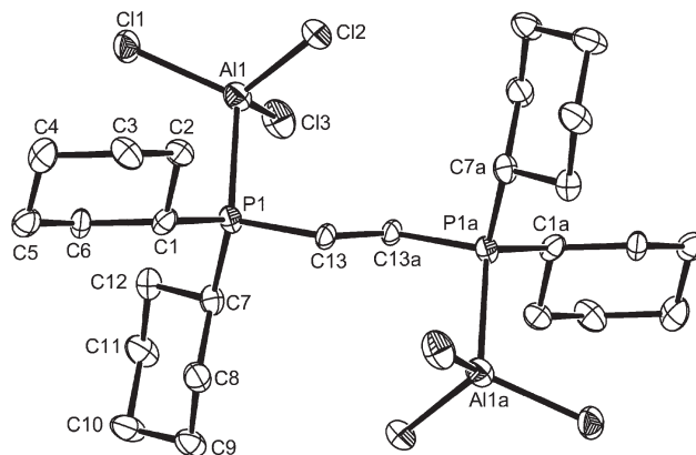
Fig. 6 The structure of centrosymmetric [(AlCl 3 ) 2 ( \mu -Cy 2 P(CH 2 ) 2 PCy 2 )] showing the atom labelling scheme. Ellipsoids are drawn at the 50% probability level and H atoms are omitted for clarity. Symmetry operation: a = 2 - x, 1 - y, 1 - z . Selected bond lengths (Å) and angles (°): Al1–Cl3 = 2.114(3), Al1–Cl1 = 2.123(3), Al1–Cl2 = 2.129(3), Al1–P1 = 2.407(3), Cl3–Al1–Cl1 = 112.98(12), Cl3–Al1–Cl2 = 113.23(12), Cl1–Al1–Cl2 = 112.00(12), Cl3–Al1–P1 = 106.20(11), Cl1–Al1–P1 = 108.76(11), Cl2–Al1–P1 = 102.90(10).
