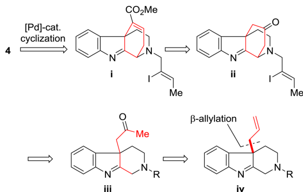
Scheme 1. Retrosynthesis of 4
