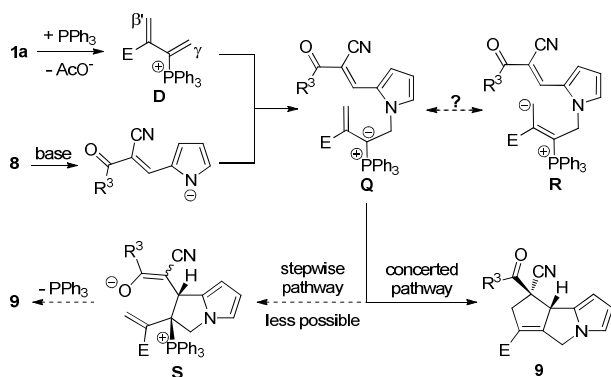
Scheme 8. Plausible Mechanism of the Reaction of 1a and 8
