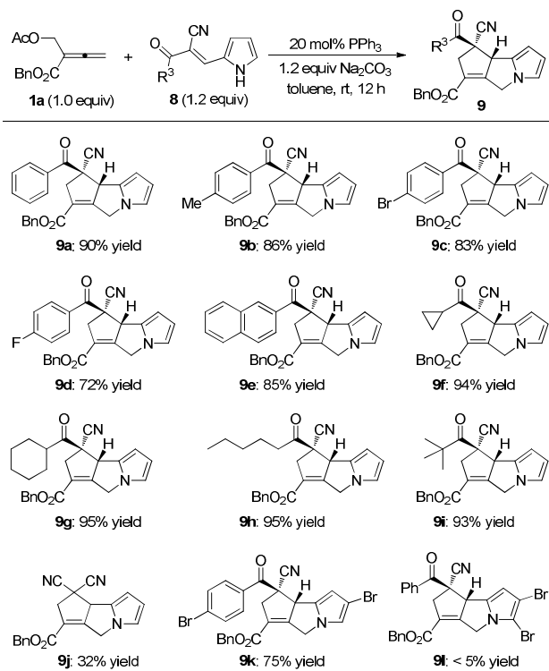
Scheme 6. Substrate scope of the \gamma -addition/[3+2] cycloaddition domino reaction. Reaction conditions: to the solution of 8 (0.24 mmol), PPh 3 (0.04 mmol) and Na 2 CO 3 (0.24 mmol) in PhMe (2 mL), was slowly added a solution of 1a (0.2 mmol) in PhMe (2 mL) over 30 minutes. Isolated yields were presented.
