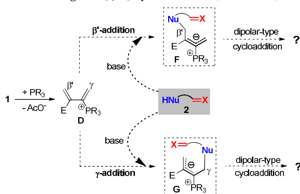
Scheme 2. Design Plan for the Addition/Cycloaddition Domino Reaction
