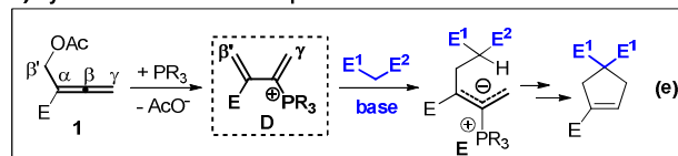
Scheme 1. Variants of the Phosphine-Catalyzed Cycloadditions of Activated Allenes
