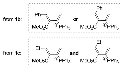
Figure 3. the Corresponding Intermediates D Derived from 1b and 1c
