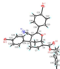
Figure 1. X-ray Structure of 30
