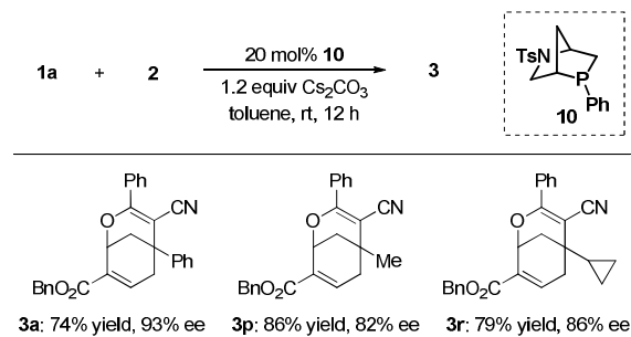
Scheme 9. Kwon's Phosphine-Catalyzed Asymmetric Reaction of 1a and 2
