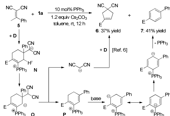
Scheme 5. The Reaction of 1a and 5
