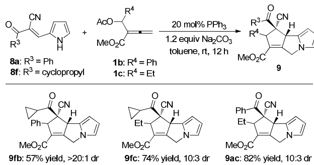
Scheme 7. Reactions of Allenolates 1b and 1c
