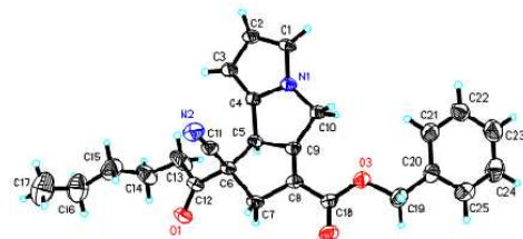
Figure 2. X-ray Structure of 9h
