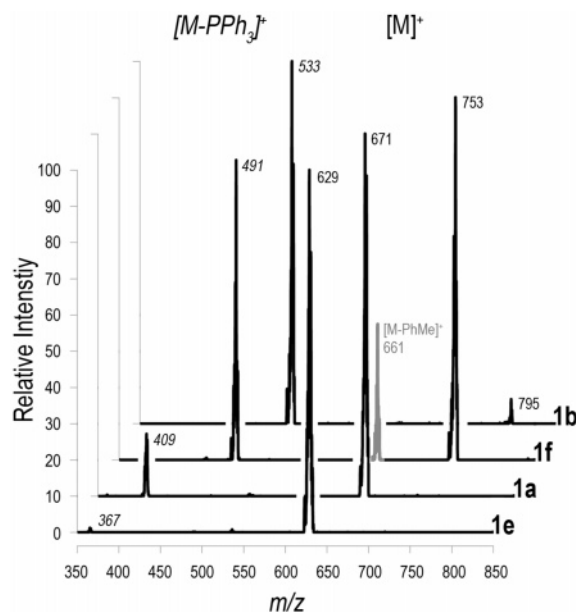
Figure 3. ESI-MS/MS of 1a , 1b , 1e , and 1f at 20% normalized collision energy [ \text{CH}_2\text{Cl}_2 , 80 °C, 5.0 kV].
