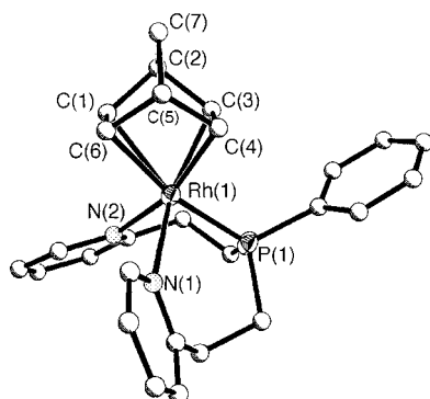
Figure 1. Molecular structure of complex 6 showing the labeling scheme. The \text{PF}_6^- anion, the molecule of \text{CH}_2\text{Cl}_2 , and all hydrogens have been omitted for clarity.
