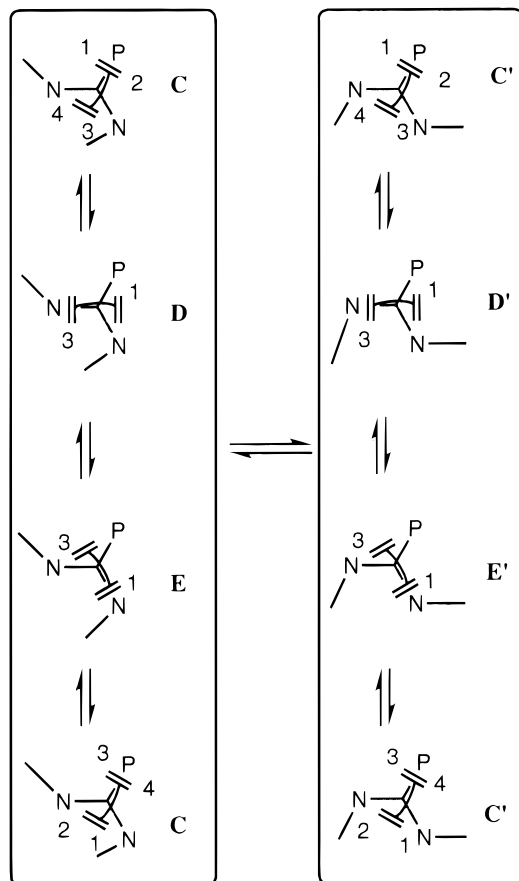
Scheme 3. Exchanges in 7 . a
