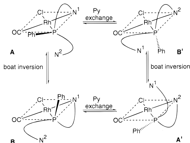
Scheme 2. Equilibrium between Two Isomers of Complex 3.
