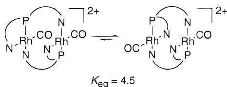
Scheme 2. Equilibrium between Two Isomers of Complex 3.
