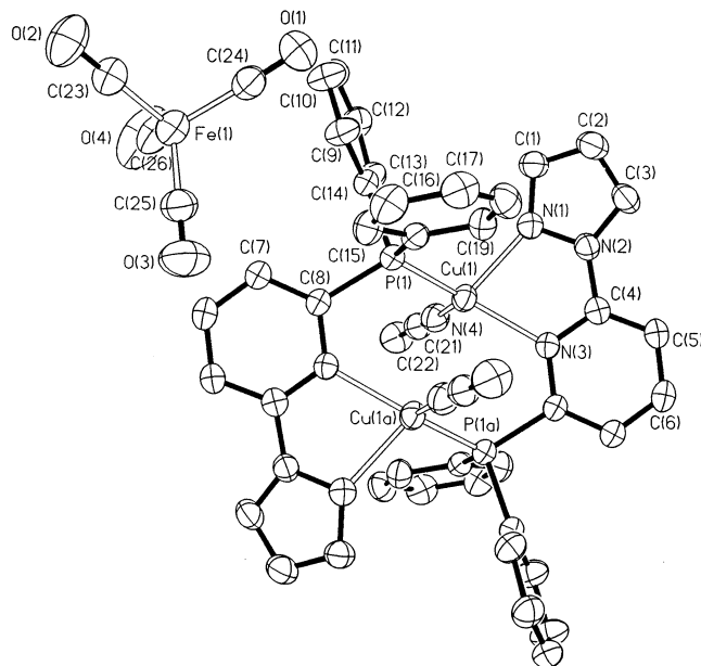
Fig. 1. Perspective view (35% thermal ellipsoids) of [\text{Cu}_2(\mu\text{-Ph}_2\text{Ppypz})_2(\text{MeCN})_2](\text{Fe}(\text{CO})_4) , 1.
