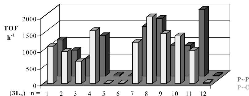
Fig. 2. Ruthenium-catalyzed hydrogenation of trans -4-phenyl-3-butene-2-one. P–P ≡ is RuCl 2 (diphos) 2 diamine, P–O ≡ RuCl 2 (ether–phosphine) 2 diamine [1]. Reaction conditions: 2-propanol, KOH as cocatalyst, T = 35 °C and P_{H_2} = 3 bar.
