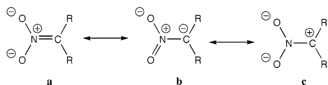
Scheme 3. Resonance Forms of the Nitromethanate Anion
