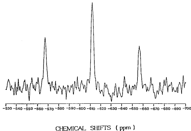
Figure 4. ^{199}\text{Hg} NMR spectrum of \text{HgBr}_2 \cdot \text{L}^2 at 298 K.
