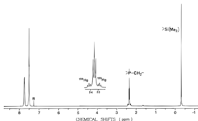
Figure 2. ^1\text{H} NMR spectrum of \text{Hg}(\text{NCS})_2 \cdot \text{L}^2 at 298 K.
