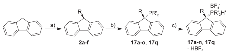
Scheme 1. Reagents and conditions: a) n\text{BuLi} , \text{RX} , \text{THF} , -60^\circ\text{C} ; b) n\text{BuLi} , \text{R}'_2\text{P-Cl} , \text{Et}_2\text{O} , -60^\circ\text{C} ; c) \text{HBF}_4\cdot\text{Et}_2\text{O} .
