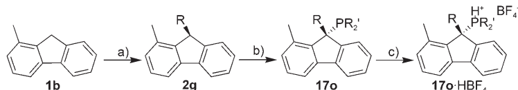
Scheme 2. Reagents and conditions: a) n\text{BuLi} , \text{EtI} ; b) n\text{BuLi} , \text{Cy}_2\text{P-Cl} ; c) \text{HBF}_4\cdot\text{Et}_2\text{O} .
