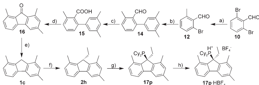
Scheme 3. Reagents and conditions: a) 1,3-propanediol, \text{ZrCl}_4 ; n\text{BuLi} , \text{MeI} , \text{H}_2\text{SO}_4 ; b) \text{Pd}(\text{OAc})_2 , \text{SIMES} , \text{Cs}_2\text{CO}_3 , 3,5- \text{Me}_2\text{-C}_6\text{H}_3\text{B}(\text{OH})_2 , dioxane; c) \text{NaClO}_2 , \text{H}_2\text{O}_2 ; d) \text{H}_2\text{SO}_4 ; e) \text{HI} , red P, propionic acid; f) n\text{BuLi} , \text{EtI} , \text{THF} , -60^\circ\text{C} ; g) n\text{BuLi} , \text{Cy}_2\text{P-Cl} , \text{Et}_2\text{O} , -60^\circ\text{C} ; h) \text{HBF}_4\cdot\text{Et}_2\text{O} .
