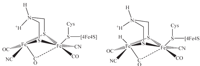
Scheme 1. Possible Intermediates in the Mechanism of Enzymatic \text{H}_2 Production by Fe-Only Hydrogenases
