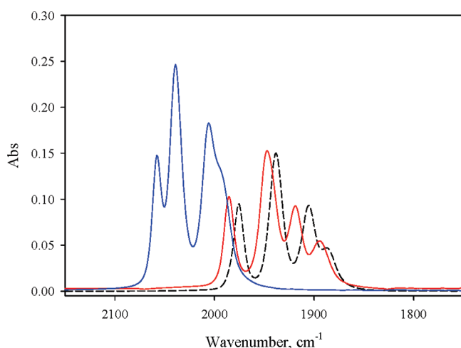
Figure 2. FTIR spectra of 1 in \text{CH}_2\text{Cl}_2 (in short dash), [\text{1-2H}^{\text{N}}]^{2+} in \text{CH}_3\text{CN} (in red), and [\text{1-2H}^{\text{N}}\text{2H}^{\text{Fe}}]^{4+} in \text{CH}_3\text{CN} (in blue).
