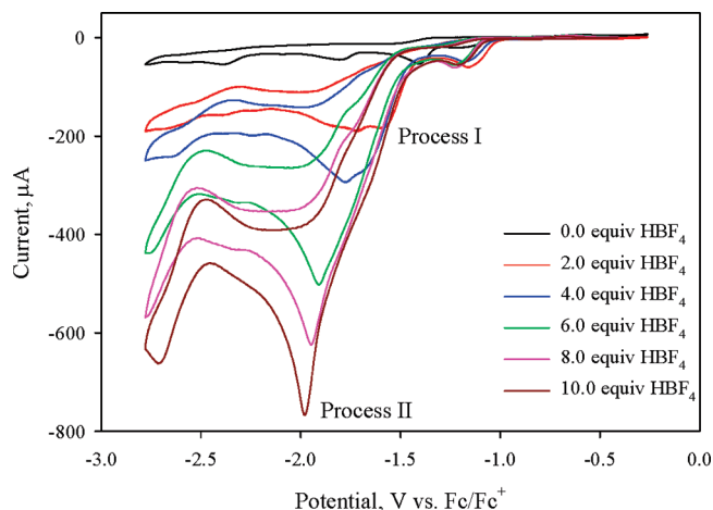
Figure 6. Cyclic voltammograms of [1-2H^N2HFe]^{4+} (1 mM) with HBF_4 in CH_3CN ( \nu = 100 \text{ mV s}^{-1} , potentials are versus Fc/Fc^+ ).
