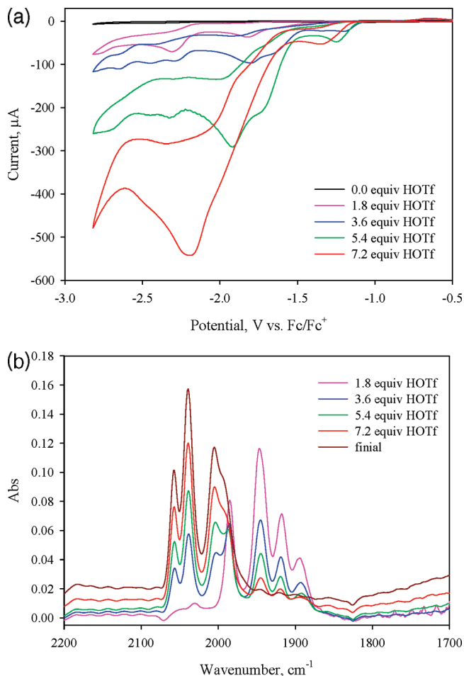
Figure 9. Cyclic voltammograms of titration of 1 (1 mM in CH_3CN ) by HOTf and their corresponding FTIR spectra.
