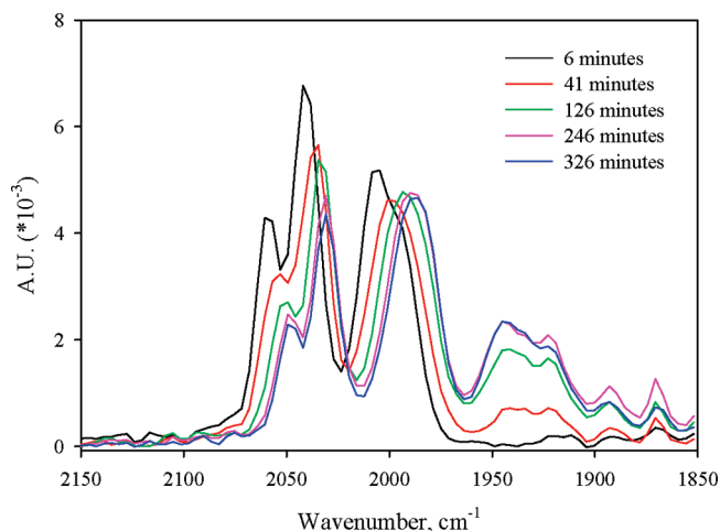
Figure 8. Spectral changes monitored by in-situ IR spectroscopy over time for [1-2H^N2HFe]^{4+} upon electrolysis at -1.35 \text{ V} in CH_3CN .
