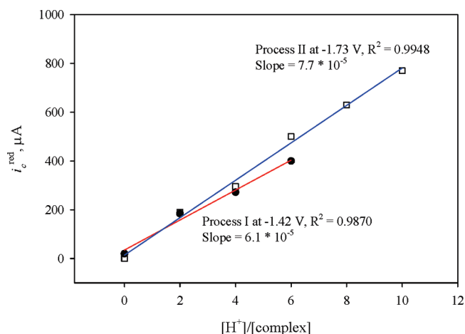
Figure 7. Dependence of current ( i_c^{\text{red}} ) vs. equivalents of HBF_4 added for [1-2H^N2HFe]^{4+} (at RT, 1 mM in CH_3CN ), where i_c^{\text{red}} is peak catalytic current.
