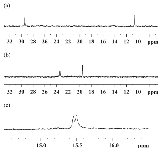
Figure 3. ^{31}\text{P} NMR spectra of (a) [\text{1-2H}^{\text{N}}]^{2+} in \text{CD}_2\text{Cl}_2 , (b) [\text{1-2H}^{\text{N}}\text{2H}^{\text{Fe}}]^{4+} in \text{CD}_2\text{Cl}_2 , and (c) High-field ^1\text{H} NMR spectrum of [\text{1-2H}^{\text{N}}\text{2H}^{\text{Fe}}]^{4+} in \text{CD}_2\text{Cl}_2 .
