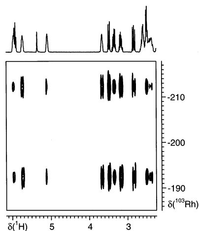
Fig. 5. Inverse ^{103}\text{Rh} spectrum for 16 showing the numerous contacts due to J(^{103}\text{Rh}, ^1\text{H}) coupling. The separation of the two horizontal cross-peaks represents the one-bond rhodium–phosphorus coupling constant. There are four strong cross-peaks in the region ca. 2.83–3.48 ppm, stemming from the four non-equivalent \text{SCH}_2 protons.
