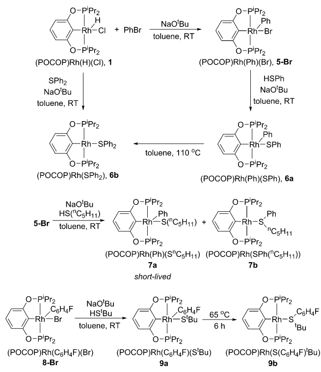
Scheme 3. Synthesis of Complexes 5–9
