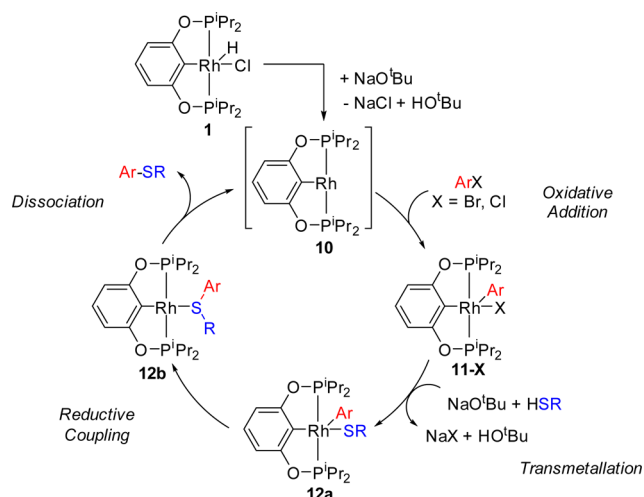
Scheme 4. Proposed Catalytic Cycle for the Coupling of Aryl Halides with Thiols Using 1 as the Catalyst
