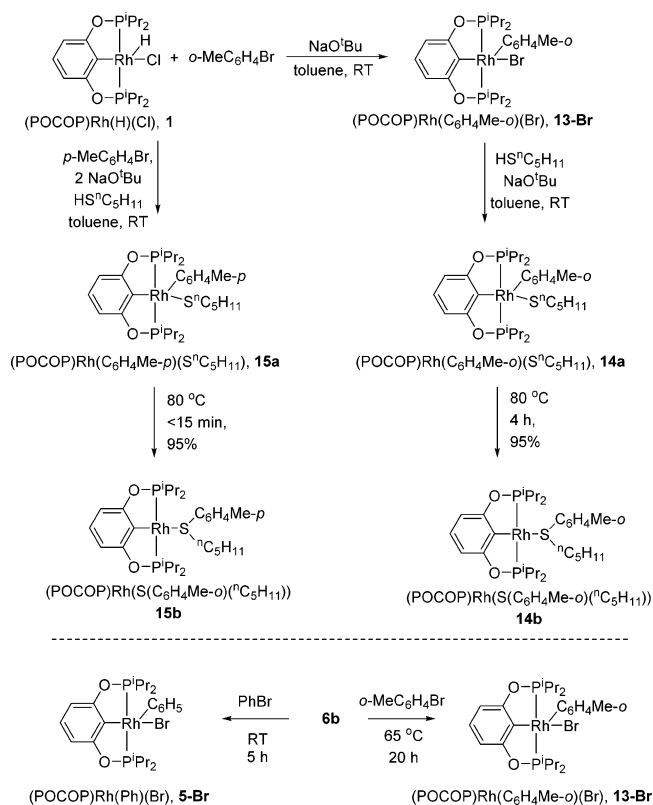
Scheme 7. Reactions Arising from o -Tolyl Halides
