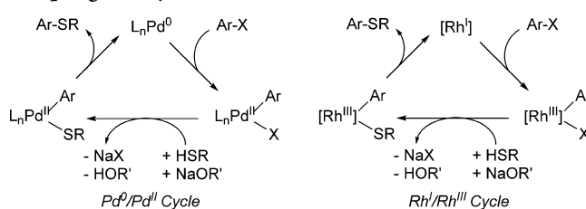
Scheme 1. General Pd 0 /Pd II and Rh I /Rh III Cycles for the Coupling of Aryl Halides with Thiols To Form Sulfides
