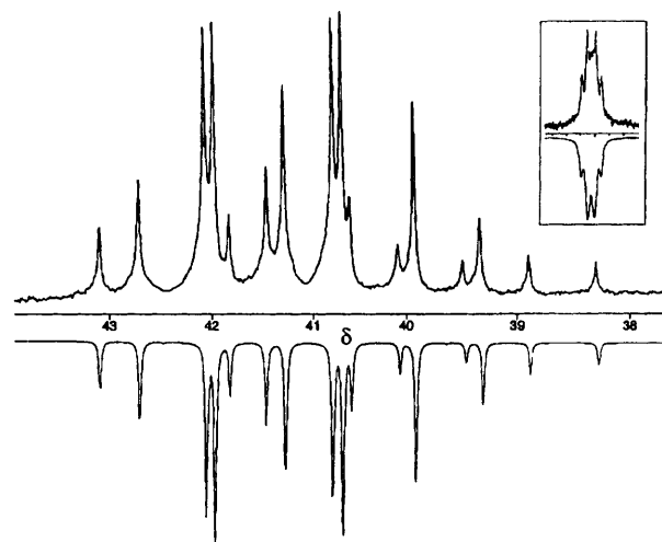
Fig. 1 Experimental (upper) and simulated (lower) ^{31}\text{P}\{-^1\text{H}\} NMR spectra of [\text{RhH}(\text{CO})(\text{PPh}_3)L^2] . The insert shows the corresponding ^1\text{H} NMR spectra in the hydride region
