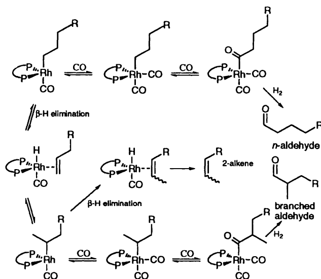
Scheme 2 Hydroformylation and isomerisation routes
