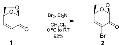
Scheme 1 Synthesis 3-bromolevoglucosenone 2
