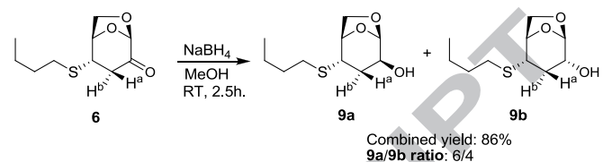
Scheme 3 Ketone reduction
