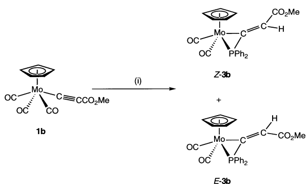
Scheme 2. Synthesis of complexes derived from [\text{CpMo}(\text{CO})_3\text{-(CCO}_2\text{Me)}] ( 1b ). Reagents and conditions: (i) \text{PPh}_2\text{H} , \text{Me}_3\text{NO} , \text{MeCN} .
