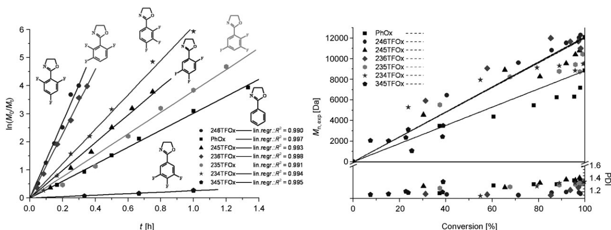
Figure 2. Polymerization of the 2-trifluorophenyl-2-oxazolines 3a–f and PhOx as a reference. Left: first-order kinetics; right: number-average molecular weight M_n against conversion.
