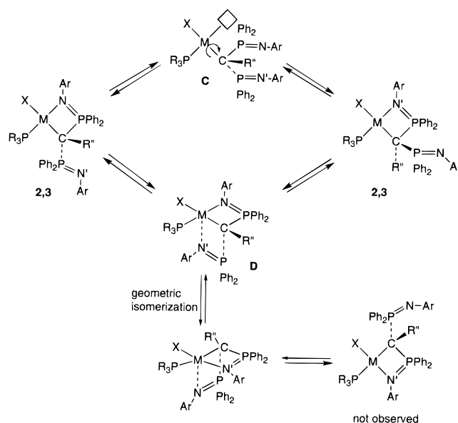
Scheme 2. N,N' Exchange in 2 and 3
