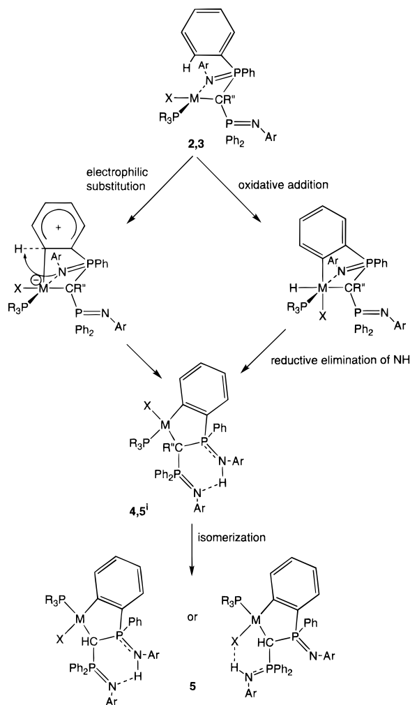
Compound 4 : M = Pt; X = Cl, Br, I; PR 3 = PEt 3 , PMe 2 Ph; R' = H. Compound 5 i and 5 : M = Pd; X = Cl; PR 3 = PEt 3 , PMe 2 Ph; R' = H.
