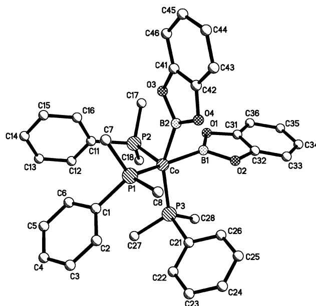
Fig. 1 A view of the molecular structure of 3 showing the atom numbering scheme. Selected bond length (Å) and angle data (°) include: Co(1)–B(1) 1.948(3), Co(1)–B(2) 1.955(3), Co(1)–P(1) 2.2237(7), Co(1)–P(2) 2.2510(7), Co(1)–P(3) 2.2067(7); B(1)–Co(1)–B(2) 71.19(12).
