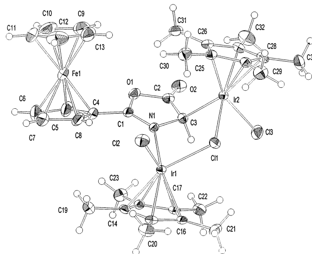
Fig. 2. Molecular structure of 19 ( \text{S}_{\text{Ir}}\text{R}_{\text{C}}\text{S}_{\text{Ir}} ) in the crystal. Selected bond lengths (Å) and angles (°): Ir(1)–N(1) 2.108(4), Ir(1)–Cl(1) 2.4320(14), Ir(2)–C(3) 2.131(5), Ir(2)–Cl(1) 2.4289(14), N(1)–C(1) 1.283(7), N(1)–C(3) 1.470(6), C(1)–C(4) 1.459(8), N(1)–Ir(1)–Cl(1) 83.84(12), Cl(2)–Ir(1)–Cl(1) 85.95(6), C(3)–Ir(2)–Cl(1) 82.32(14), Cl(3)–Ir(2)–Cl(1) 87.91(6), Ir(2)–Cl(1)–Ir(1) 110.19(5), C(1)–N(1)–C(3) 107.8(4), C(1)–N(1)–Ir(1) 134.5(4), N(1)–C(1)–C(4) 131.9(5), C(2)–C(3)–Ir(2) 115.8(4), N(1)–C(3)–Ir(2) 115.6(3), N(1)–Ir(1)–C(11)–Ir(2) –8.44(0.12), C(3)–N(1)–C(1)–O(1) 2.07(0.59), N(1)–C(1)–C(4)–C(8) 29.93(1.04), Ir(1)–N(1)–C(3)–Ir(2) –72.29(0.38).
