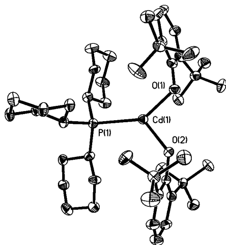
Figure 1. Thermal ellipsoid representation of \text{Cd}(\text{O}-2,6\text{-}^i\text{Bu}_2\text{C}_6\text{H}_3)_2 \cdot \text{PCy}_3 , complex 1 .
