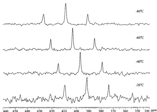
Figure 8. Temperature-dependent ^{113}\text{Cd} NMR spectra of \text{Cd}(\text{O-2,6-Ph}_2\text{C}_6\text{H}_3)_2 \cdot 2\text{P}^n\text{Bu}_3 .
