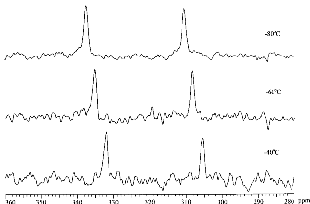
Figure 6. Temperature-dependent ^{113}\text{Cd} NMR spectra of \text{Cd}(\text{O-2,6-Ph}_2\text{C}_6\text{H}_3)_2 \cdot \text{P}^n\text{Bu}_3 .
