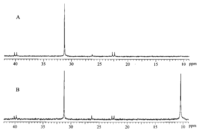
Figure 3. ^{31}\text{P} NMR spectra of complex 1 . (A) in \text{C}_6\text{D}_6 . (B) In \text{C}_6\text{D}_6 with 1 equiv of added \text{PCy}_3 .
