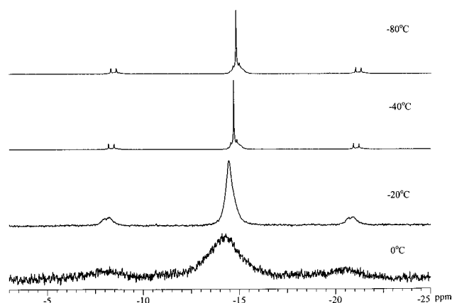
Figure 7. Temperature-dependent ^{31}\text{P} NMR spectra of \text{Cd}(\text{O-2,6-Ph}_2\text{C}_6\text{H}_3)_2 \cdot 2\text{P}^n\text{Bu}_3 .
