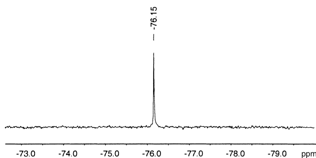
Fig. 2. Partial ^{31}\text{P} -NMR spectrum ( (\text{D}_6) acetone, 162 MHz) of 8·3b
