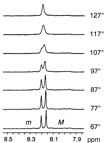
Fig. 8. Variable-temperature ^1\text{H} -NMR measurements (400 MHz, (\text{D}_6)\text{DMSO} ) of 6c . H–C(3') signal of the major ( M ) and minor ( m ) diastereoisomeric conformations \delta and \lambda^2 .
