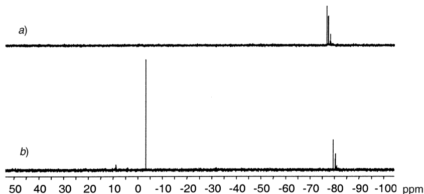
Fig. 11. Partial ^{31}\text{P} -NMR spectrum (162 MHz, DMSO) of salt 8·3a a) before and b) after heating at 147^\circ
