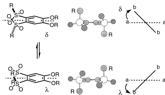
Fig. 4. Views of the conformations adopted by ortho-positioned sulfonyl groups and configurational assignment ( \delta and \lambda ). a \cdots a constitutes the plane of the phenyl ring, and b \cdots b represents the line passing through the R substituents.
