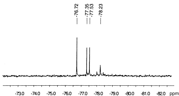
Fig. 3. Partial ^{31}\text{P} -NMR spectrum ( (\text{D}_6) DMSO; 162 MHz) of 8·3a
