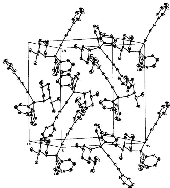
Fig. 3. Cell packing diagram of \text{Au}(\text{C}\equiv\text{CPh})(\text{nmdpp}) ( 2 ).
