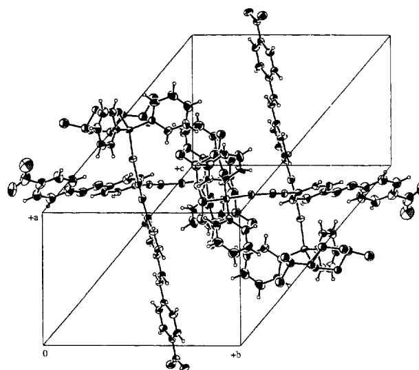
Fig. 4. Cell packing diagram of \text{Au}((E)\text{-}4,4'\text{-C}\equiv\text{CC}_6\text{H}_4\text{CH}=\text{CHC}_6\text{H}_4\text{NO}_2)(\text{nmdpp}) ( 5 ).
