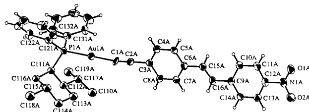
Fig. 2. Molecular structure and atomic labelling scheme for one of the molecules of Au(( E )-4,4'-C≡CC 6 H 4 CH=CHC 6 H 4 NO 2 )(nmdpp) ( 5 ). 20% thermal ellipsoids are shown for the non-hydrogen atoms; hydrogen atoms have arbitrary radii.
