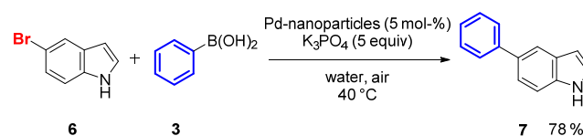
Scheme 2. Suzuki-Miyaura cross-coupling of 5-bromoindole ( 6 ) and phenylboronic acid ( 3 ) catalyzed by ligand-free solvent-stabilized Pd-nanoparticles (Pd-NP).
