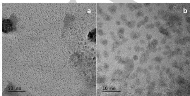
Figure 1. (a) Transmission electron microscopy (TEM) image of suspended solvent-stabilized Pd-nanoparticles; (b) Fivefold magnification.
