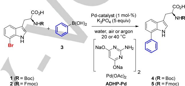
Scheme 1. SUZUKI-MIYAUURA reaction of N α -protected L-7-bromotryptophan with both biocompatible ADHP-Pd and solvent-stabilized Pd-nanoparticles.
