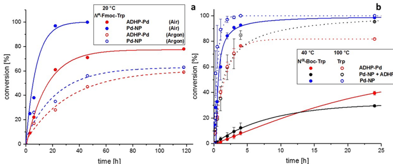
Figure 2. Conversion as function of time in the Suzuki-Miyaura reaction (a) of N ε -Fmoc-L-7-bromotryptophan (20 °C) and phenylboronic acid catalysed by ADHP-Pd (red) or Pd nanoparticles (Pd-NP) (blue) under aerobic or inert conditions and (b) of N α -Boc-L-7-bromotryptophan (40 °C) or unprotected L-7-bromotryptophan (100 °C) and phenylboronic acid catalysed by ADHP-Pd (red), Pd-NP (blue) or Pd-NP + ADHP (grey).
