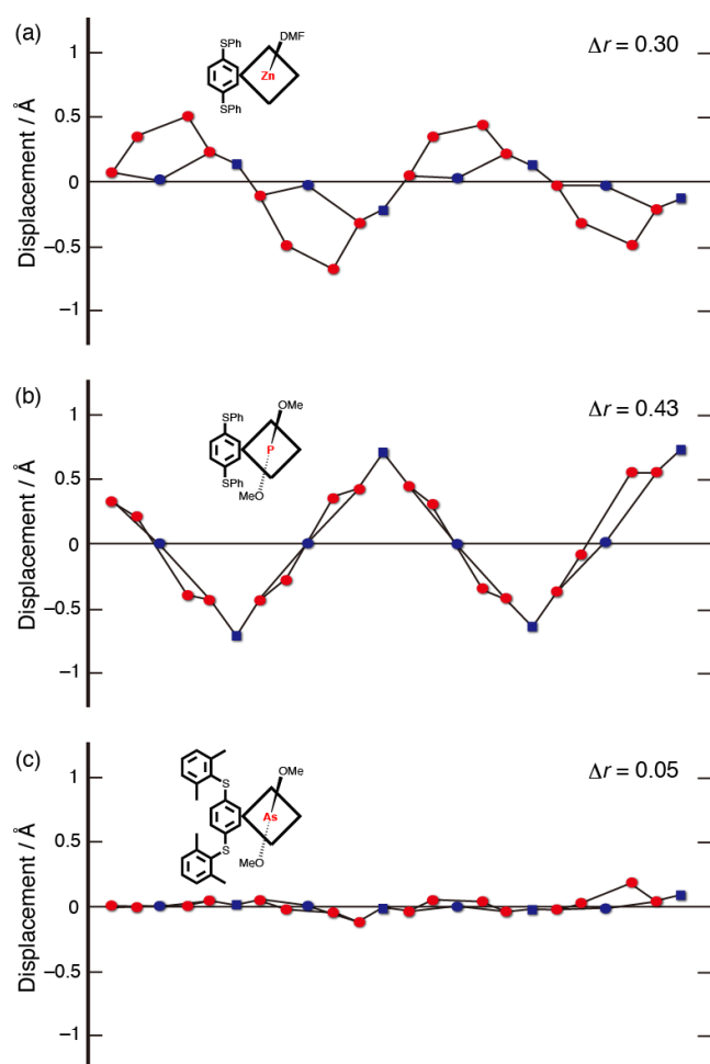
Figure 9. Views of the skeletal deviation of the atoms from the 4N mean plane for (a) 5•DMF , (b) 4a , and (c) 8 . Red circles indicate carbon atoms. Blue squares and circles indicate nitrogen atoms at meso -positions and coordinating nitrogen atoms, respectively.
