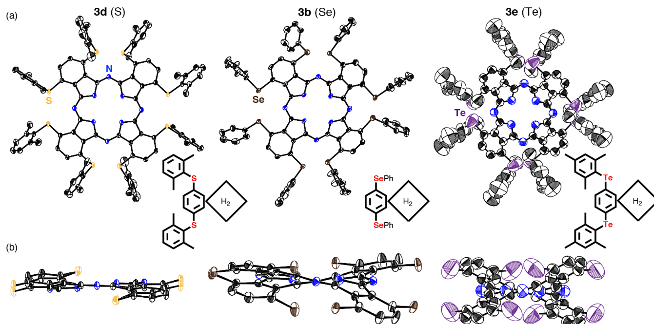
Figure 3. X-ray crystal structure of 3b , 3d , and 3e . The thermal ellipsoids were scaled to the 50% probability level. (a) top view; (b) side view (peripheral substituents omitted). H atoms, and the solvent molecule have been omitted for clarity.
