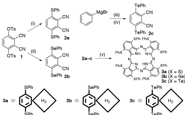
Scheme 2. Synthesis of \alpha -chalcogenyl free-base Pcs a
