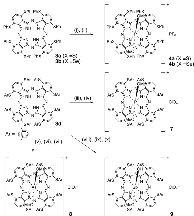
Scheme 3. Synthesis of Pc complexes with group 15 elements a
