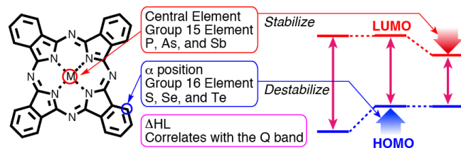
Scheme 1. Molecular design of Near-IR absorbing Pcs.
