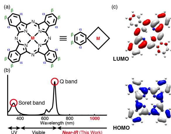
Figure 1. (a) Molecular structure of Pc. (b) Typical absorption spectrum of a metallated Pc with D_{4h} symmetry. (c) Frontier orbitals of an unsubstituted free-base Pc.
