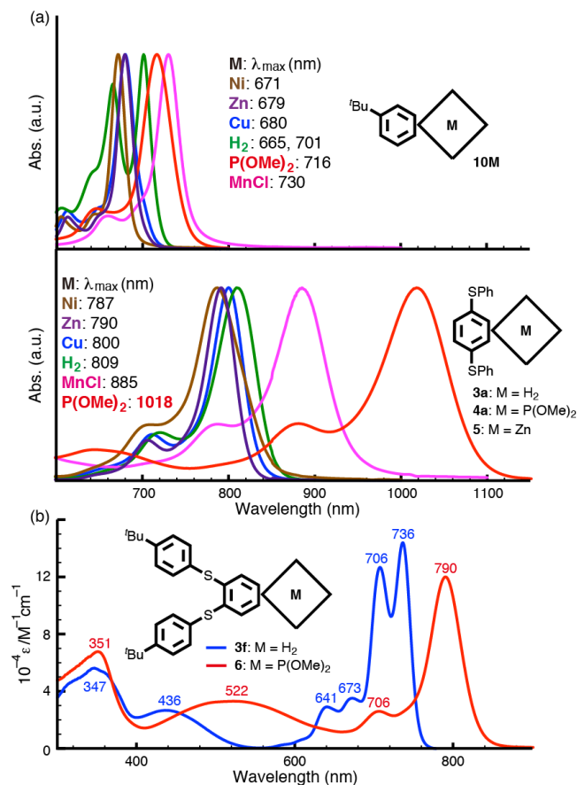
Figure 5. (a) Absorption spectra of metallated and phosphorus(V) complexes of \beta - t -Bu 4 Pc (top) and those of \alpha -(PhS) 8 Pc (bottom) in CHCl 3 . (b) Absorption spectra of free-base \beta -(thioaryl) 8 Pc 3f (blue) and \beta -(thioaryl) 8 PcP(OMe) 2 , i.e. 6 (red) in CHCl 3 . In (a), the intensity was normalized at the Q band.
