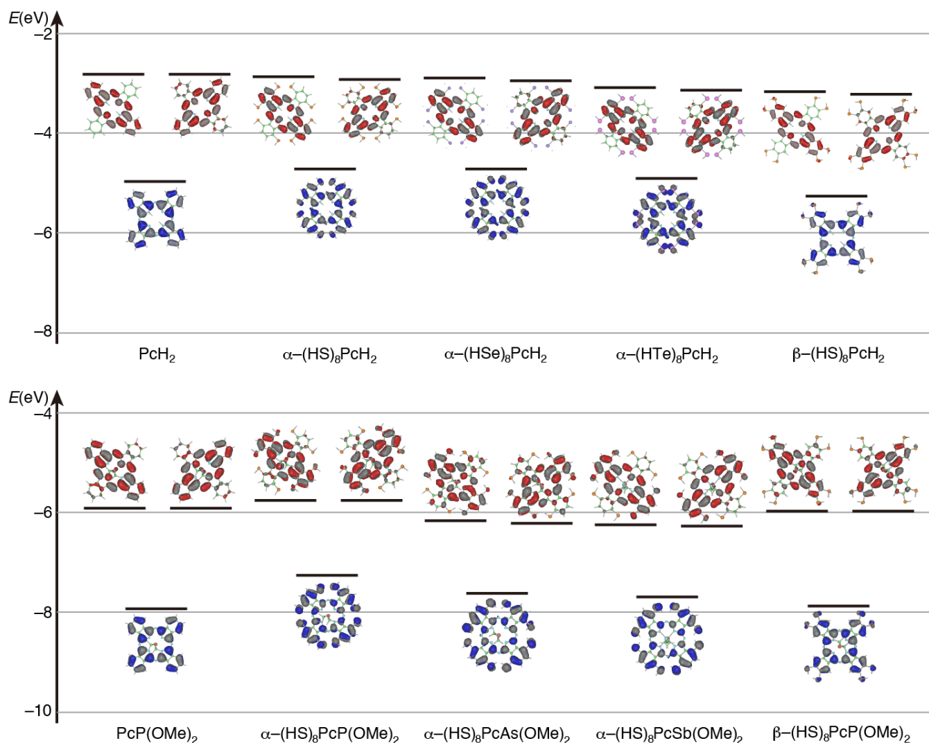
Figure 12. Energy levels of frontier MOs and their contour plots obtained from calculations. Blue and red plots indicate occupied and unoccupied MOs, respectively. Calculations were performed at the B3LYP/6-31G* level (for details, see the SI).
