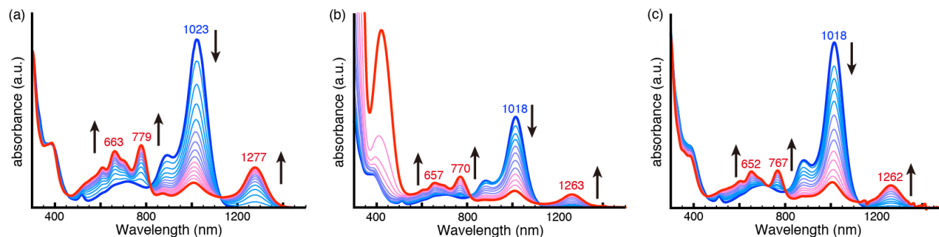
Figure 11. Spectral changes of 8 solution by (a) applying -0.2 V potential vs Ag/AgCl reference electrode in o\text{-DCB} , (b) adding \text{Me}_{10}\text{Fc} in \text{CH}_2\text{Cl}_2 , and (c) adding triethylamine in \text{CH}_2\text{Cl}_2 .
