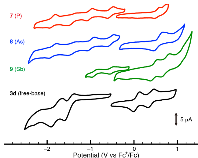
Figure 10. Cyclic voltammetry data for 3d , and 7-9 . Cyclic voltammograms were acquired from 1.0 mM solutions of analyte in 0.1 M n\text{Bu}_4\text{NClO}_4/o\text{-DCB} . Ferrocene was used as an internal standard and set to 0 V.
