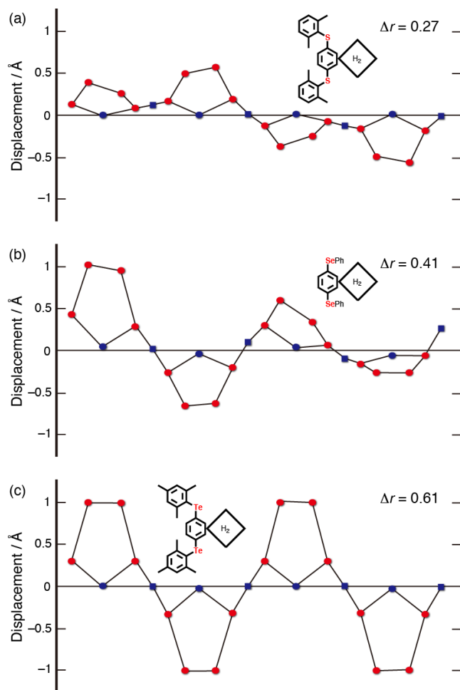
Figure 4. Views of the skeletal deviation of the atoms from the 4N mean plane for (a) 3d , (b) 3b , and (c) 3e . Red circles indicate carbon atoms. Blue squares and circles indicate nitrogen atoms at meso -positions and coordinating nitrogen atoms, respectively.
