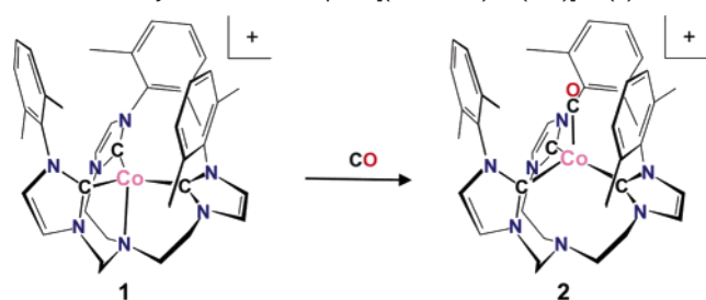
Scheme 2. Synthesis of Complex [(\text{TIMEN}^{\text{xy}})\text{Co}(\text{CO})]\text{Cl} ( 2 )
