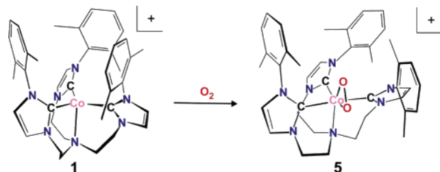
Scheme 4. Synthesis of Peroxo Complex [(TIMEN xy )Co(O 2 )]BPh 4 (5)
