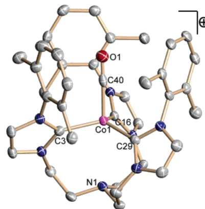
Figure 2. Solid-state molecular structure of [(\text{TIMEN}^{\text{xy}})\text{Co}(\text{CO})]\text{Cl}\cdot 2\text{CH}_3\text{CN} ( 2\cdot 2\text{CH}_3\text{CN} ). Hydrogen atoms, anion, and solvent molecules are omitted for clarity; thermal ellipsoids are shown at 50% probability. Selected bond lengths (angstroms) and angles (degrees): Co(1)–C(3) 2.0347(17) , Co(1)–C(16) 2.0545(17) , Co(1)–C(29) 2.0267(16) , Co(1)–C(40) 1.8463(19) , Co(1)–N(1) 3.034 , C(40)–O(1) 1.103(2) , C(3)–Co(1)–C(16) 117.92(6) , C(3)–Co(1)–C(29) 113.02(6) , C(16)–Co(1)–C(29) 118.33(6) .
