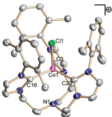
Figure 3. Solid-state molecular structure of [(TIMEN yl )Co(Cl)]Cl·DMSO ( 3 ·DMSO). Hydrogen atoms, anion, and solvent molecules are omitted for clarity; thermal ellipsoids are shown at 50% probability. Selected bond lengths (angstroms) and angles (degrees): Co(1)–C(3) 2.078(5), Co(1)–C(16) 2.080(5), Co(1)–C(29) 2.074(5), Co(1)–Cl(1) 2.2557(15), Co(1)–N(1) 3.061, C(3)–Co(1)–C(16) 117.57(19), C(3)–Co(1)–C(29) 114.50(19), C(16)–Co(1)–C(29) 114.4(2).
