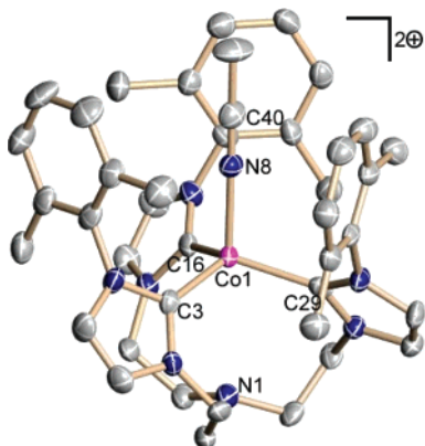
Figure 4. Solid-state molecular structure of [(TIMEN yl )Co(CH 3 CN)](BPh 4 ) 2 ·CH 3 CN ( 4 ·CH 3 CN). Hydrogen atoms, anions, and solvent molecules are omitted for clarity; thermal ellipsoids are shown at 50% probability. Selected bond lengths (angstroms) and angles (degrees): Co(1)–C(3) 2.028(3), Co(1)–C(16) 2.033(3), Co(1)–C(29) 2.047(3), Co(1)–N(8) 2.035(3), Co(1)–N(1) 3.146, C(3)–Co(1)–C(16) 111.71(13), C(3)–Co(1)–C(29) 111.53(13), C(16)–Co(1)–C(29) 121.24(13), Co(1)–N(1)–C(40) 179.1(3).
