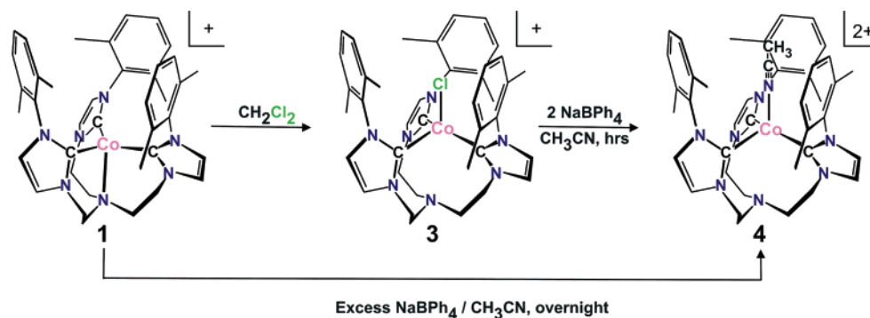
Scheme 3. Synthesis of Complexes [(\text{TIMEN}^{\text{xy}})\text{Co}(\text{Cl})]\text{Cl} ( 3 ) and [(\text{TIMEN}^{\text{xy}})\text{Co}(\text{CH}_3\text{CN})](\text{BPh}_4)_2 ( 4 )
