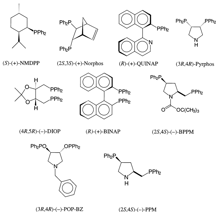
Fig. 2. Selected phosphine ligands (see Table 1).
