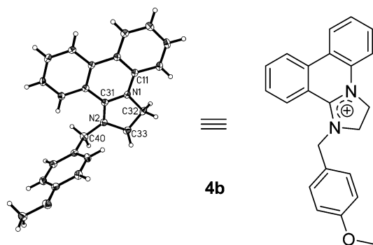
Figure 2. ORTEP representation of structure 4b . Selected bond lengths showing delocalization of charge [Å]: N1–C31 1.340(3), N2–C31 1.333(3), N2–C33 1.472(3), N1–C32 1.475(3), N2–C40 1.457(3), N1–C11 1.389(3).
