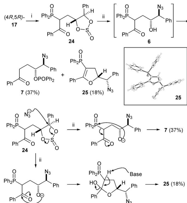
Scheme 6 Reagents and conditions: i) \text{SOCl}_2 , pyridine, \text{CH}_2\text{Cl}_2 , 47%; ii) \text{NaN}_3 , DMF, 60 °C. Inset: X-ray crystal structure of azide 25 with ellipsoids at 50% probability.
