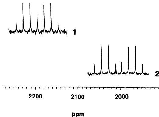
Fig. 4. ^{199}\text{Hg}\{^1\text{H}\} -NMR spectra ( \text{CD}_2\text{Cl}_2 , 223K) of 1 and 2 .
