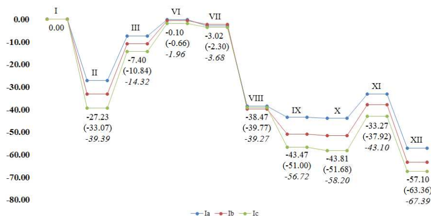
Figure 1 Potential Energy Surface (based on \Delta G values) for the formation of 2b from 1b by using cyanamide ( Ia ), methylcyanamide ( Ib ) and phenylcyanamide ( Ic ). Y-axis represents the relative free energy changes in kcal/mol.
