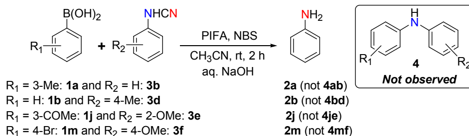
Scheme 4 Reactions with Arylcyanamides and Arylboronic acids Mediated by PIFA-NBS
