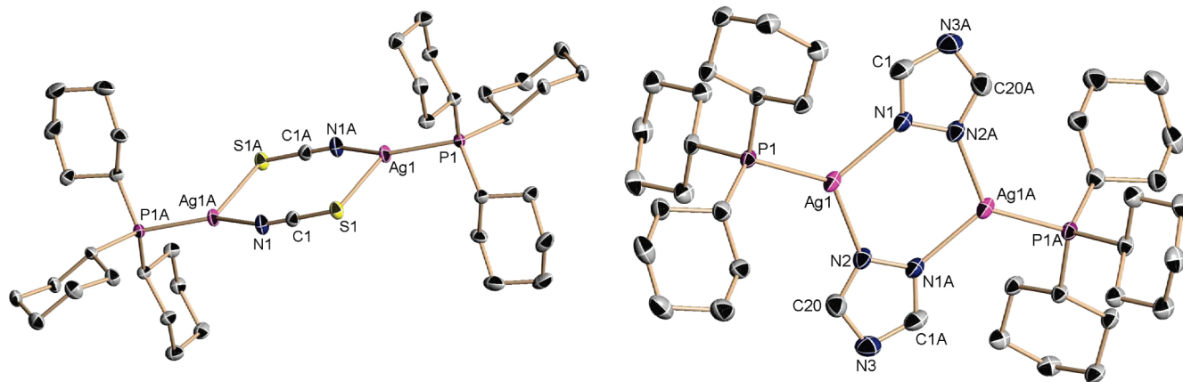
Figure 4. ORTEP representation of one crystallographically independent molecule of 4 (left) and 5 showing 50% probability ellipsoids and partial atom-labeling scheme; hydrogen atoms (for 4 and 5 ) have been omitted for clarity. Selected bond distances (Å) and bond angles (deg): ( 4 ) Ag1–N1, 2.131(3); Ag1–P1, 2.3588(7); Ag1–S1, 2.6720(8); C1–N1, 1.151(4); N1–Ag1–P1, 151.84(7); N1–Ag1–S1, 101.36(7); P1–Ag1–S1, 106.71(2); N1–C1–S1, 179.5(3). ( 5 ) Ag1–N1, 2.2594(19); Ag1–N2, 2.2093(18); Ag1–P1, 2.3654(5); N1–Ag1–N2, 107.01(7); N1–Ag1–P1, 120.71(5); N2–Ag1–P1, 132.07(5).
