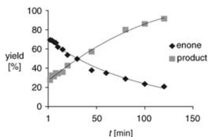
Figure 1. Kinetic curves for the continuous conversion of enone into 3-alkylketone catalyzed by phosphorous acid diamide monoester 6b and \text{Cu}(\text{OTf})_2 . (GC analysis commenced after 1 min, when \text{ZnEt}_2 addition was complete. Cyclohexanone was used as the internal standard, added stoichiometrically to the reaction mixture simultaneously with the enone).
