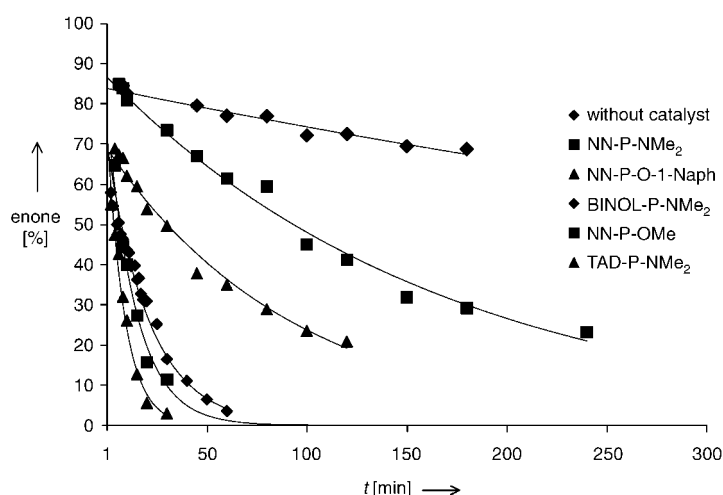
Figure 2. Kinetics of the conjugate ethylation of cyclohexenone by dialkylzinc catalyzed by \text{Cu}^{\text{I}} complexes of various \text{P}^{\text{III}} ligands, monitored as decreasing enone concentration (GC analysis, the first injection was only carried out after complete addition of diethylzinc and therefore does not start at 100 %).
