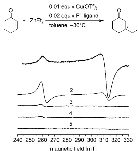
Scheme 3. Top: Standard reaction protocol for the kinetic investigations. Bottom: EPR spectra of 1 , free \text{Cu}(\text{OTf})_2 with [\text{Cu}(\text{OTf})_2] = 4.2 \text{ mM} in toluene; 2 , \text{Cu}(\text{OTf})_2 :ligand 8 (1:2); 3 , \text{Cu}(\text{OTf})_2 :ligand 8 (1:2) with a 24-fold excess of \text{ZnEt}_2 in toluene after 6 min; 4 , after 10 min; 5 , after 18 min (300 K).
